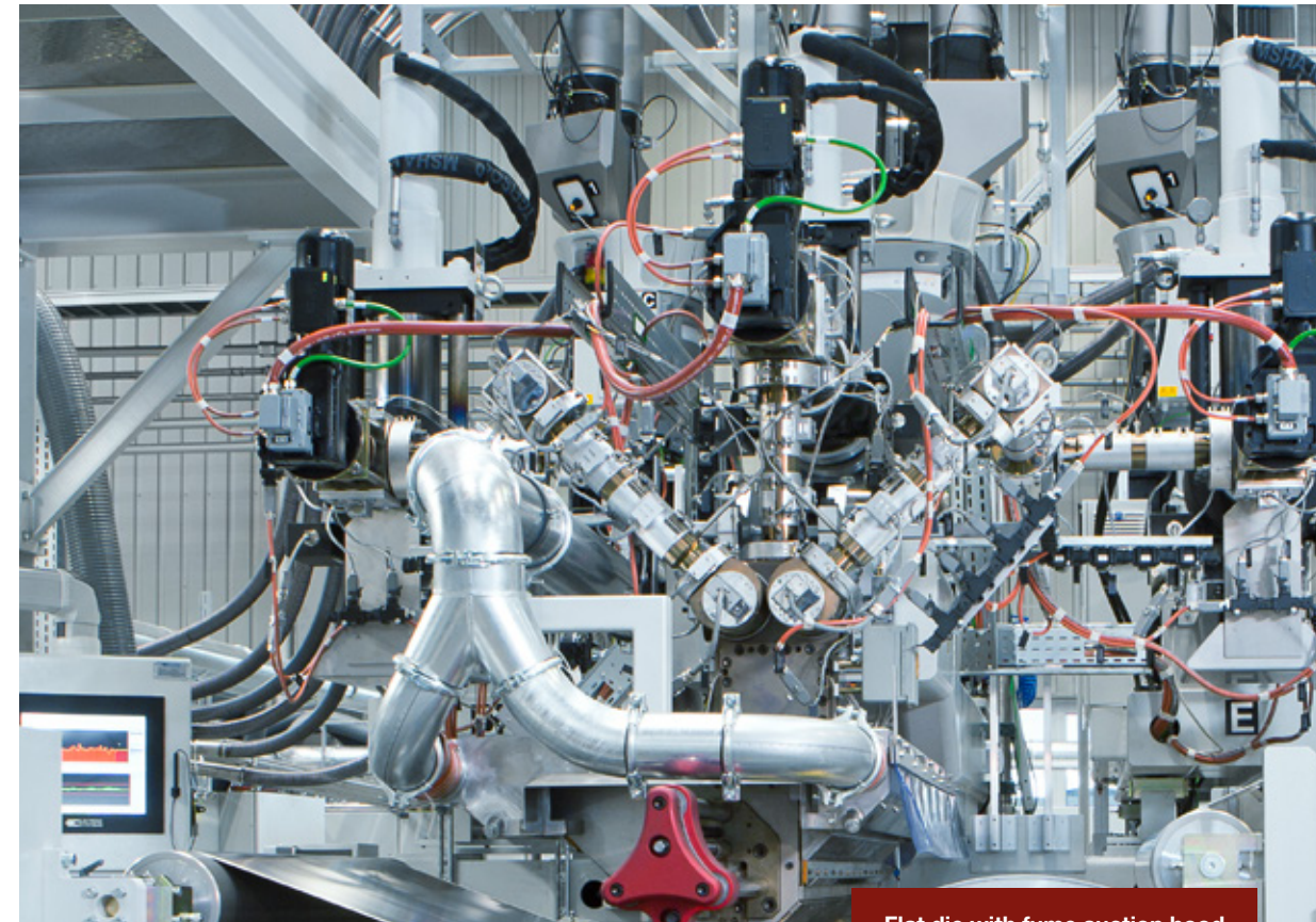
Flat die with fume suction hood
